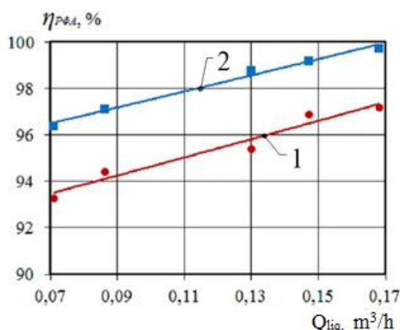
Figure 6. Cleaning efficiency RFA fluid consumption of Q_{liq} depending on
