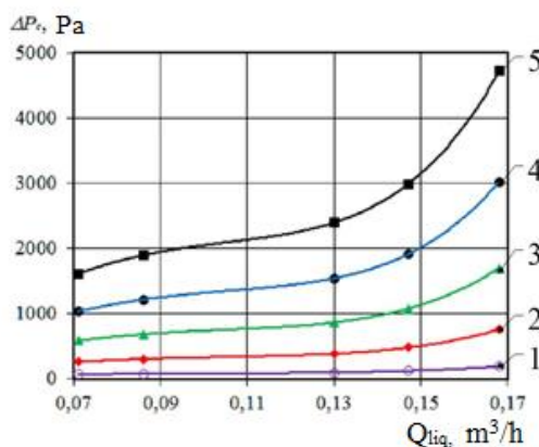
1 – v_g=5 m/s; 1 – v_g=10 m/s; 1 – v_g=15 m/s; 1 – v_g=20 m/s; 1 – v_g=25 m/s. Figure 4. a= 45^\circ va \rho_g=1.89 kg/m 3 hydraulic resistance DP_s dependence of liquid consumption Q_{liq}
