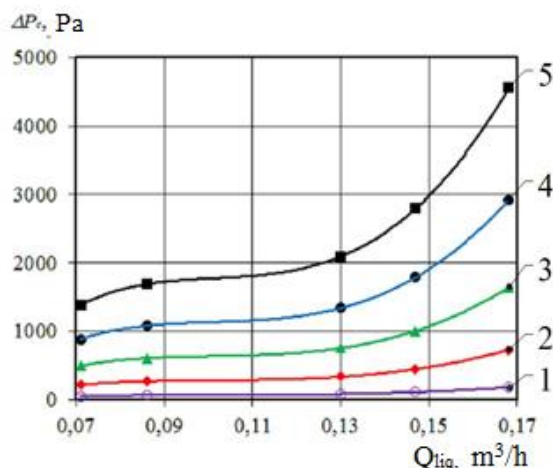
1 – v g =5 m/s; 2 – v g =10 m/s; 3 – v g =15 m/s; 4 – v g =20 m/s; 5 – v g =25 m/s. Figure 5. a= 60° va ρ g =1.89 kg/m 3 hydraulic resistance Dependence of fluid consumption Q liq
