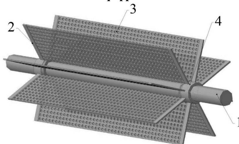
Figure 1. Scheme of the device equipped with a surface contact element.
