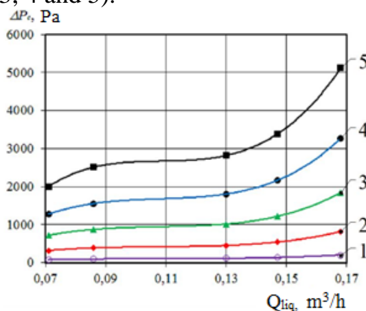
1 – v_g=5 m/s; 1 – v_g=10 m/s; 1 – v_g=15 m/s; 1 – v_g=20 m/s; 1 – v_g=25 m/s. Figure 3. a= 30^\circ and \rho_g=1.89 kg/m 3 Dependence of hydraulic resistance DP_s on liquid consumption Q_{liq} at
