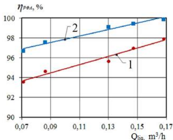
Figure 7. Cleaning efficiency RFA fluid consumption of Q_{liq} depending on
