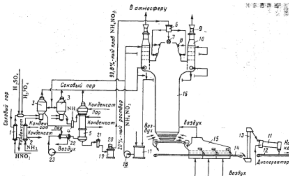
Fig. 1. Scheme of AS-72 ammonium nitrate unit:
