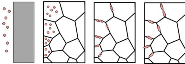
Fig.2.- Adsorbing a hydrogen gas into steel of the metal.
