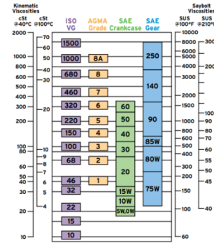
Fig.3. Comparative viscosity chart.
